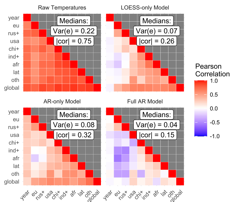
Figure C3. Correlation in the model errors across regions. The four subplots represent different models, within which each row and column describes residuals for a region, or the numerical year ('year'), or the global GMST model ('global'). The cells are colored by the Pearson correlation of these residuals. Each subplot also reports the median variance of the model errors ('Var(e)') across regions, and the median absolute value of the correlation of all off-diagonal correlations ('|cor|'). The 'Raw Temperatures' subplot treats all variation in temperatures as model error; the 'LOESS-only Model' subplot regresses region temperatures on a smoothed GMST; the 'AR-only Model' subplot regresses region temperatures on delayed temperatures; and the 'Full AR Model' includes both regressors.
