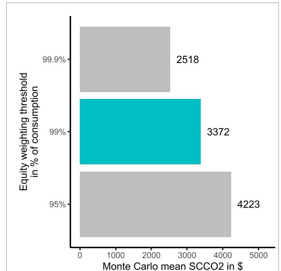
Figure B1. Mean SCCO 2 based on 50 000 Monte Carlo under different equity-weighting thresholds for SSP2-4.5. The blue bar marks our default setting.
