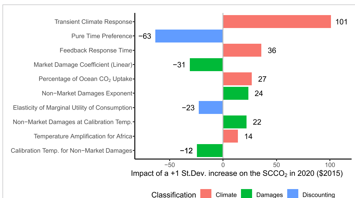
Figure A3. Impact of a parameter increase by one standard deviation on the 2020 SCCO 2 based on the default PAGE-ICE model for SSP2-4.5 (deterministic run). The SCCO 2 impact is calculated as the difference between the SCCO 2 for the mean of the respective parameter's Monte Carlo distribution, and the SCCO 2 for a parameter value equal to the mean value increased by one standard deviation, while all other parameters remain at their default value. Only parameters with an absolute SCCO 2 impact of at least $10 are displayed here.
