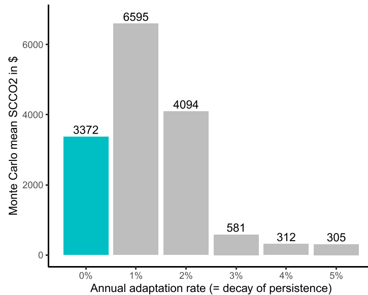
Figure B9. Mean SCCO 2 based on 50 000 Monte Carlo under different annual decay rates of damage persistence for SSP2-4.5. The blue bar marks our default setting of zero decay, (i.e. damage persistence remains constant over time).
