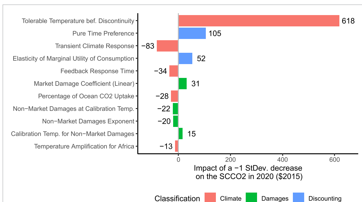
Figure A4. Impact of a parameter decrease by one standard deviation on the 2020 SCCO 2 based on the default PAGE-ICE model for SSP2-4.5 (deterministic run). The SCCO 2 impact is calculated as the difference between the SCCO 2 for the mean of the respective parameter's Monte Carlo distribution, and the SCCO 2 for a parameter value equal to the mean value increased by one standard deviation, while all other parameters remain at their default value. Only parameters with an absolute SCCO 2 impact of at least $10 are displayed here. Note that a one standard deviation decrease in the tolerable temperature before a discontinuity occurs triggers the discontinuity in this particular case, thus leading to a substantial increase in the SCCO 2 .
